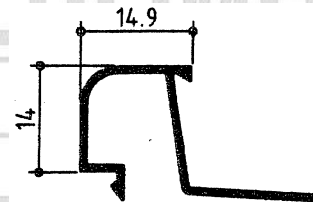
Junq. Clim Curvo
