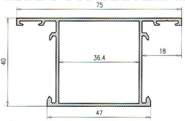
Pilastra 40*40 09
