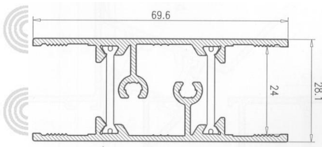
Parteluz Climalit PRT
