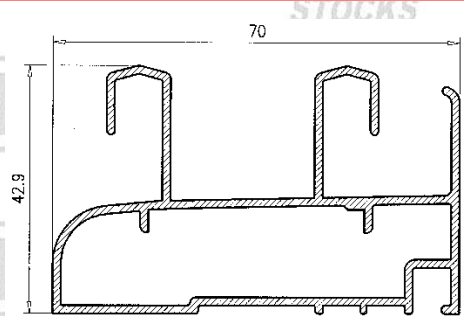
Marco 3 carriles 18202
