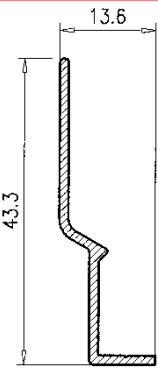
Visera Superior 18807
