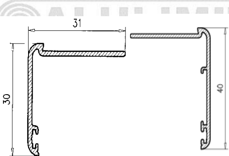
Visera Superior 18807
