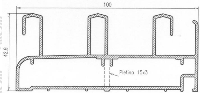
Marco 3 carriles 18202
