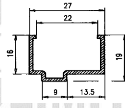
U Climalit 198
