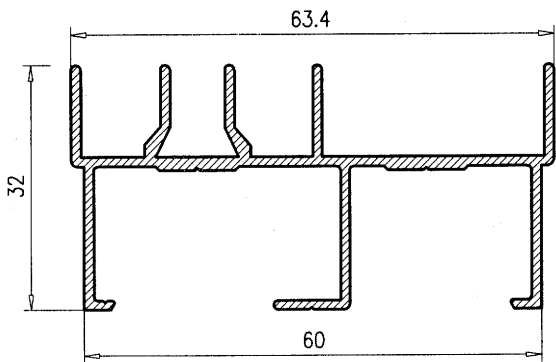
Marco Lateral
