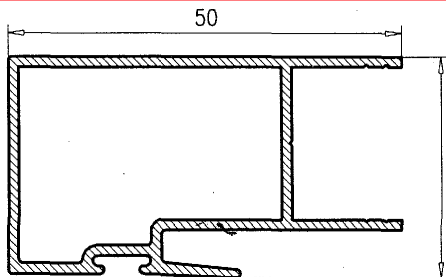
Hoja Central Climalit 50 7013
