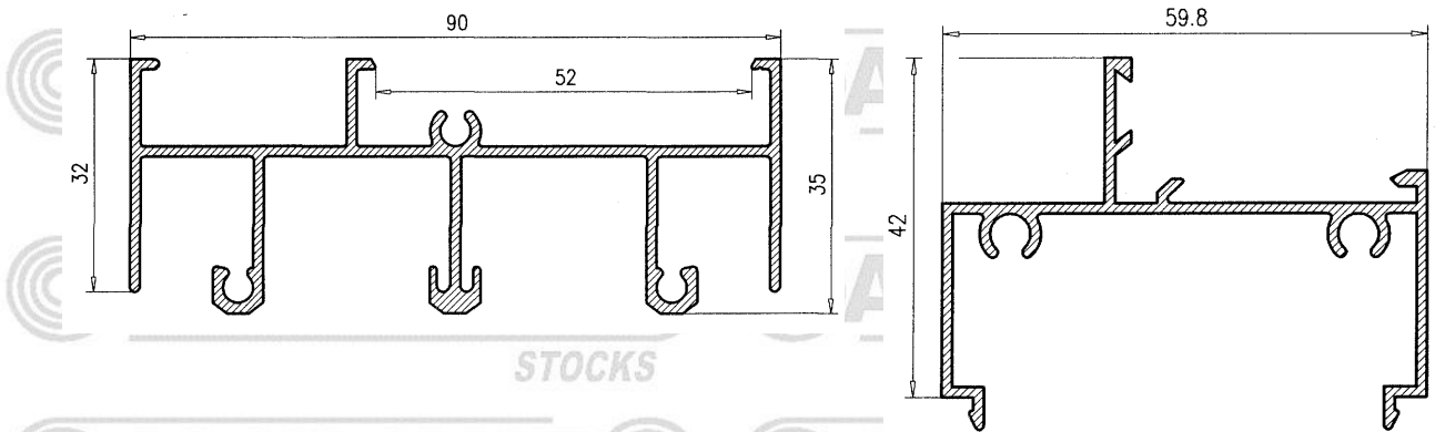
Marco Superior 3 carriles
