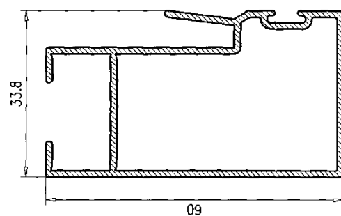
Hoja Central Normal 60 124347
