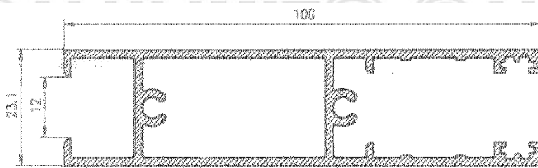
Hoja Central Climalit 60 124346
