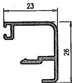
Junq. base 23 h- 27.5 36261
