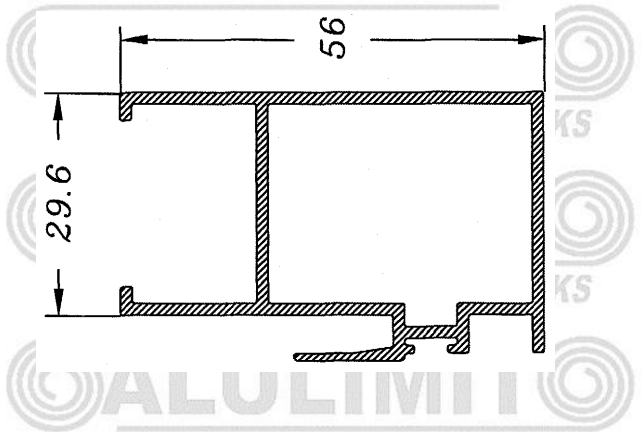
Hoja Central Climalit 835
