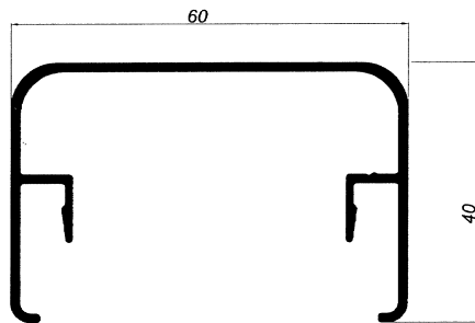
Pasamano Rectangular 60*40
