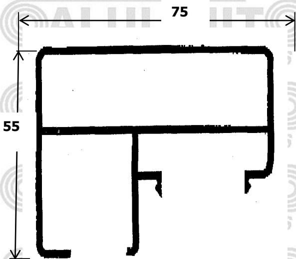
Pasamano Cristal 324 STOCKS
