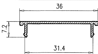
Grapa
