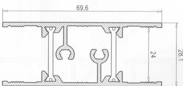
Parteluz Climalit PRT
