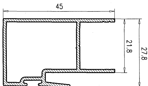
Hoja Central Climalit 45
