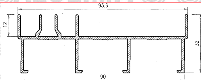
Marco Lateral 3 carriles
