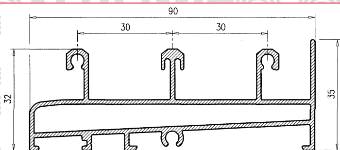
Marco Superior 3 carriles
