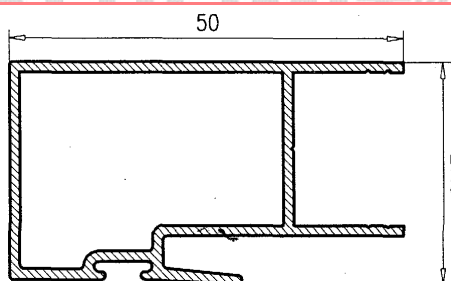
Hoja Central Climalit 50
