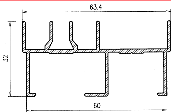
Marco Lateral
