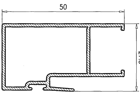
Hoja Central 50 c/16
