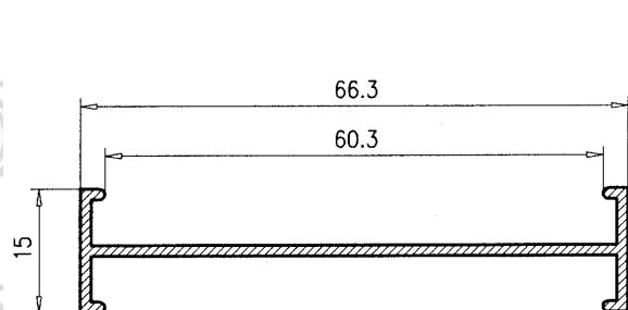
Union 60
