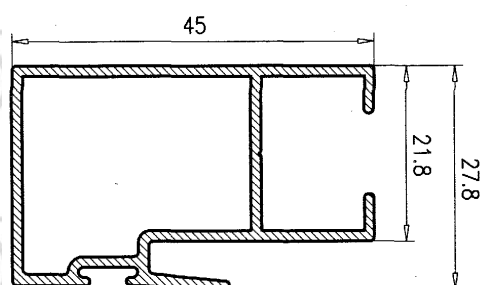
Hoja Central 45
