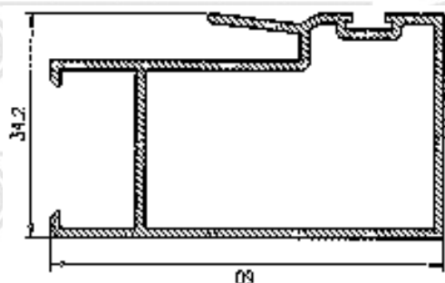
Hoja Central Climalit 60
