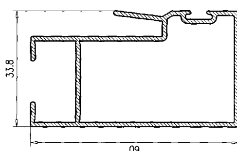
Hoja Central Normal 60
