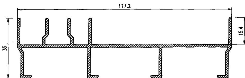
Marco Lateral 3 carriles
