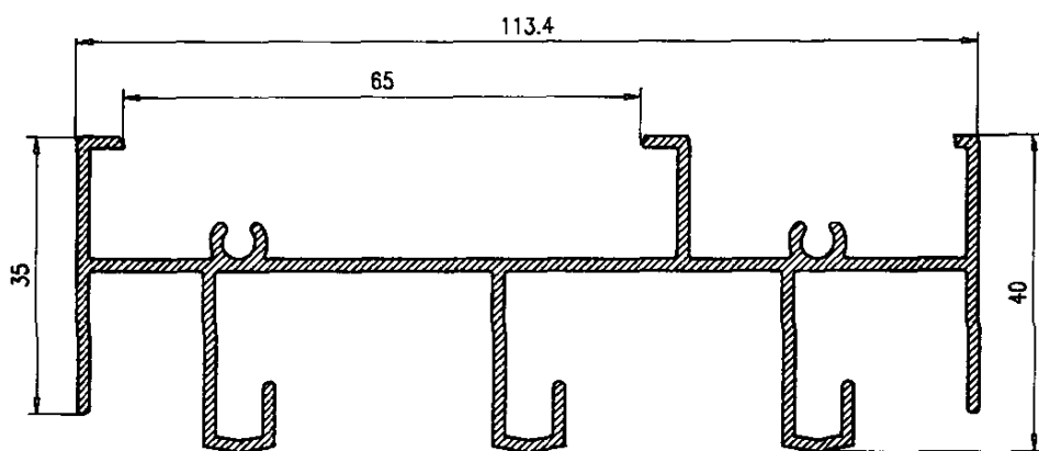
Marco Superior 3 carriles
