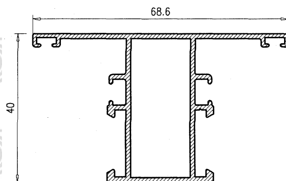
Pilastra Ventana 128580
