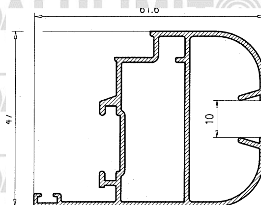
Inversor Curvo 128385
