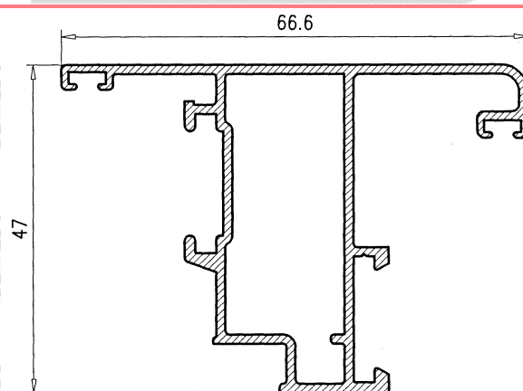
Pilastra Ventana 128580
