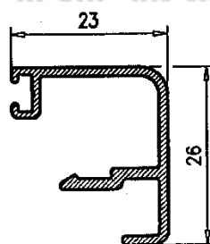
Junq. base 23 h- 27.5
