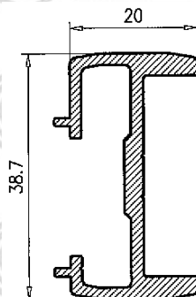
Marco Lateral 62
