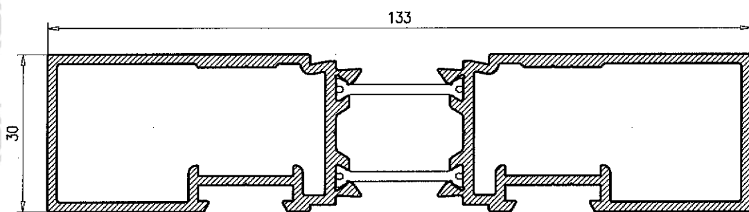
Marco Lateral 62
