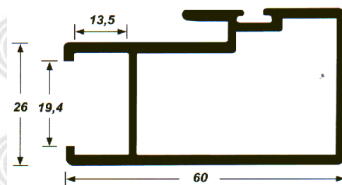
Hoja Central Climalit 7213
