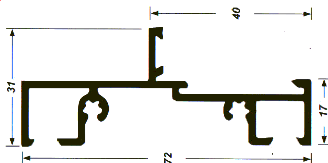
Hoja Central Climalit 7213
