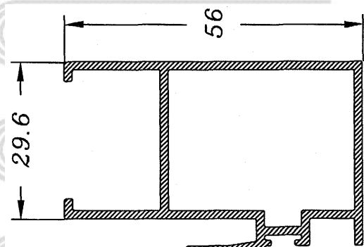
Hoja Central Climalit 835
