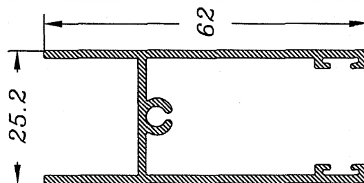
Hoja Central Climalit 835
