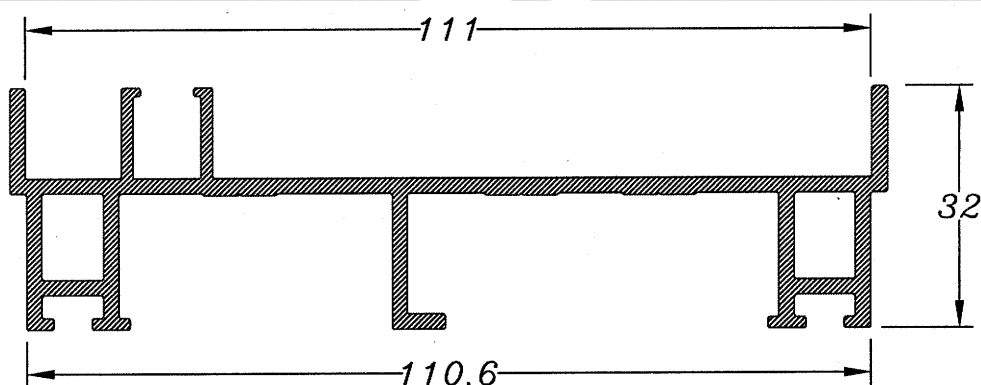
Marco Lateral 3 carriles 823
