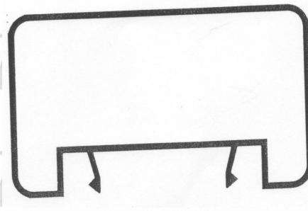
Pasamano Rectangular 70*40
