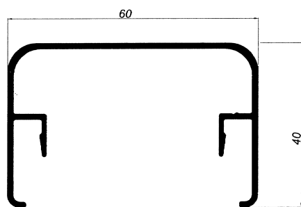
Pasamano Rectangular 60*40
